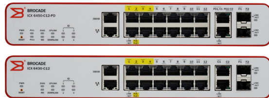
Figure 2: The Brocade ICX 6430-C and 6450-C Compact Switches support two 1 GbE RJ-45 and two 1 GbE SFP ports for uplink and 12 1 GbE RJ-45 ports with four PoE/PoE+ capable ports in a compact and fanless design—ideal for deployment outside the wiring closet. The Brocade ICX 6450-C can be powered either from its internal power supply or with PoE/PoE+ through its two RJ45 uplink ports, enabling the switch to be deployed in environments where no AC power outlet is present.
