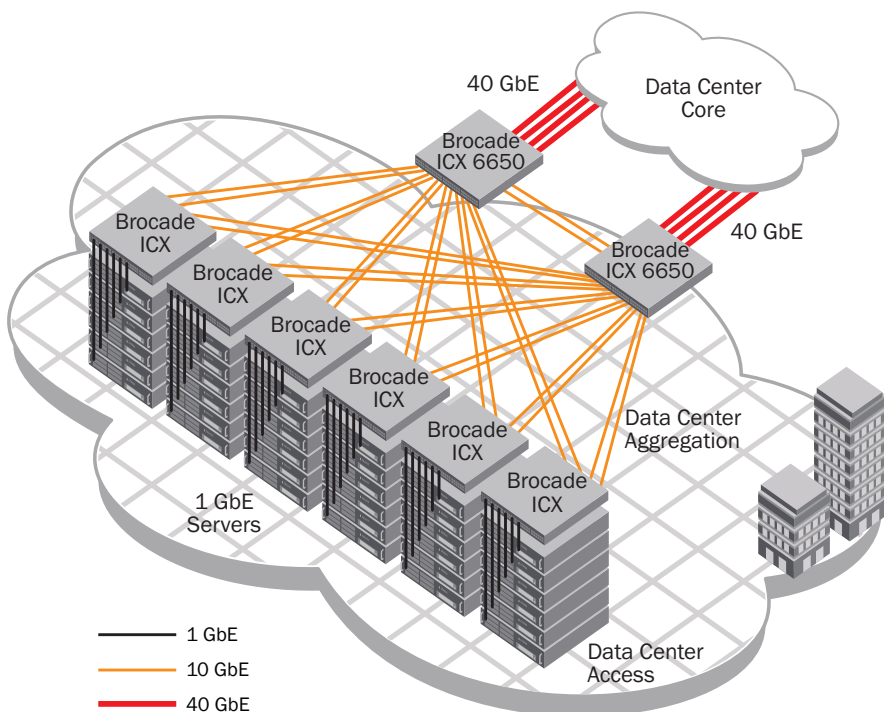
Figure 5: Brocade ICX 6430 and 6450 Switches provide ToR access while Brocade ICX 7750 Switches provide data center aggregation.
